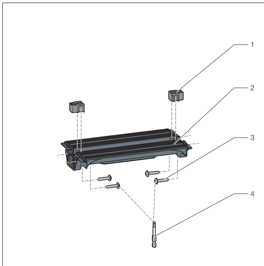
Fig. 2: connection piece, scope of delivery
