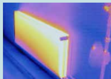
Folosind XStream
